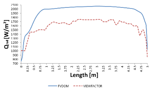
Figure 8. Radiation heat transfer on the mat for the different radiation models.
