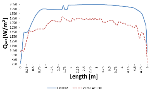
Figure 10. Net heat transfer on the mat for the different radiation models.
