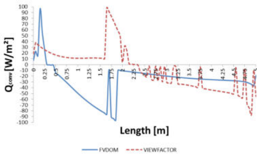
Figure 9. Convection heat transfer on the mat for the different radiation models.
