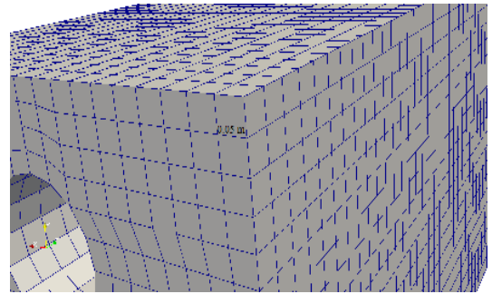
Figure 7. Isometric view of the computational mesh.
