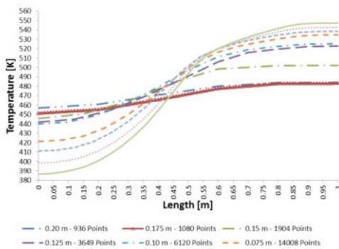
Figure 5. Temperature fields in the center of the mat for t=3600 s.
