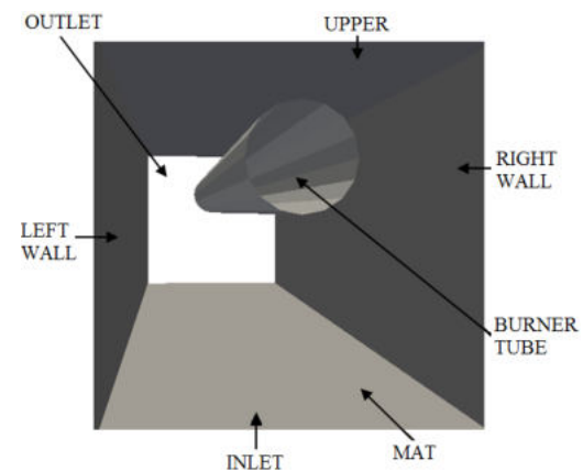
Figure 3. Schematic drawing of furnace-isometric view.
