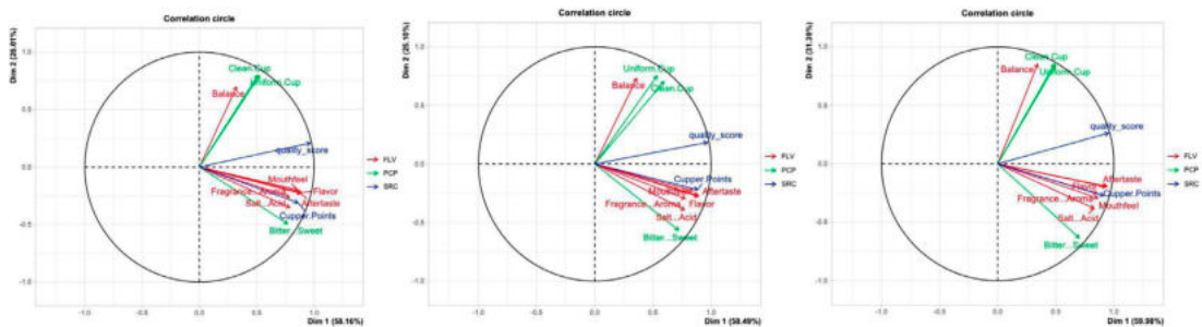
Figure 6. Correlation circle representing the projection of the input variables and the output variable in the imputed dataset with 30, 35, and 45 missing values presence.
